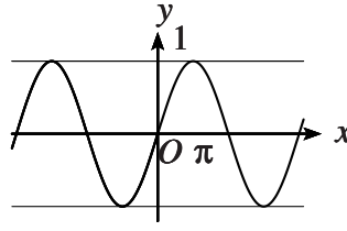
FIGURE 6 – Le graphe de \sin
