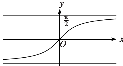
FIGURE 11 – Le graphe de arctan
