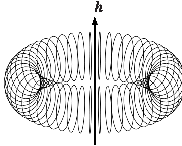
FIGURE 48 – Tore
