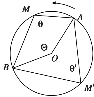
FIGURE 54 – Points cocycliques
